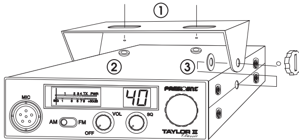
MOUNTING DIAGRAM
